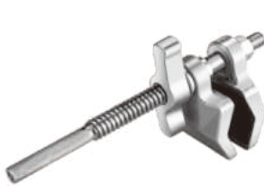
W033 Can be clamped: 15–60mm Weight : 0.3kg Size: 181x98x72mm
