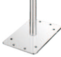
MF1672 6" baby wall plate Weight : 0.58kg Size: 80x150x154mm Joint: \varnothing 16mm
