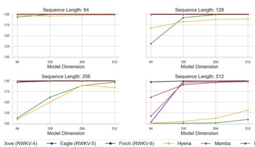
e 4: MQAR tasks. An increase in sequence length correlates with increased task difficulty
