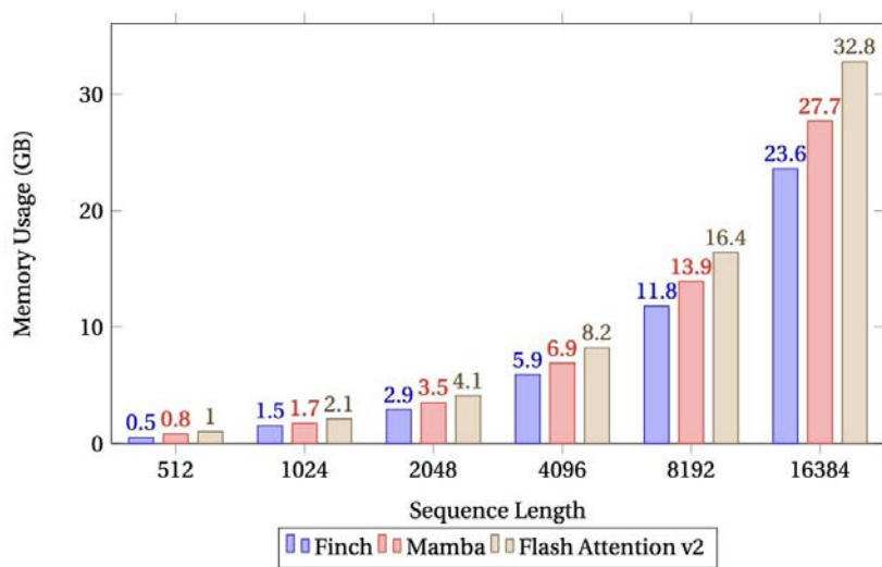
Figure 6: Memory Usage vs. Sequence Length (A100 80GB)
